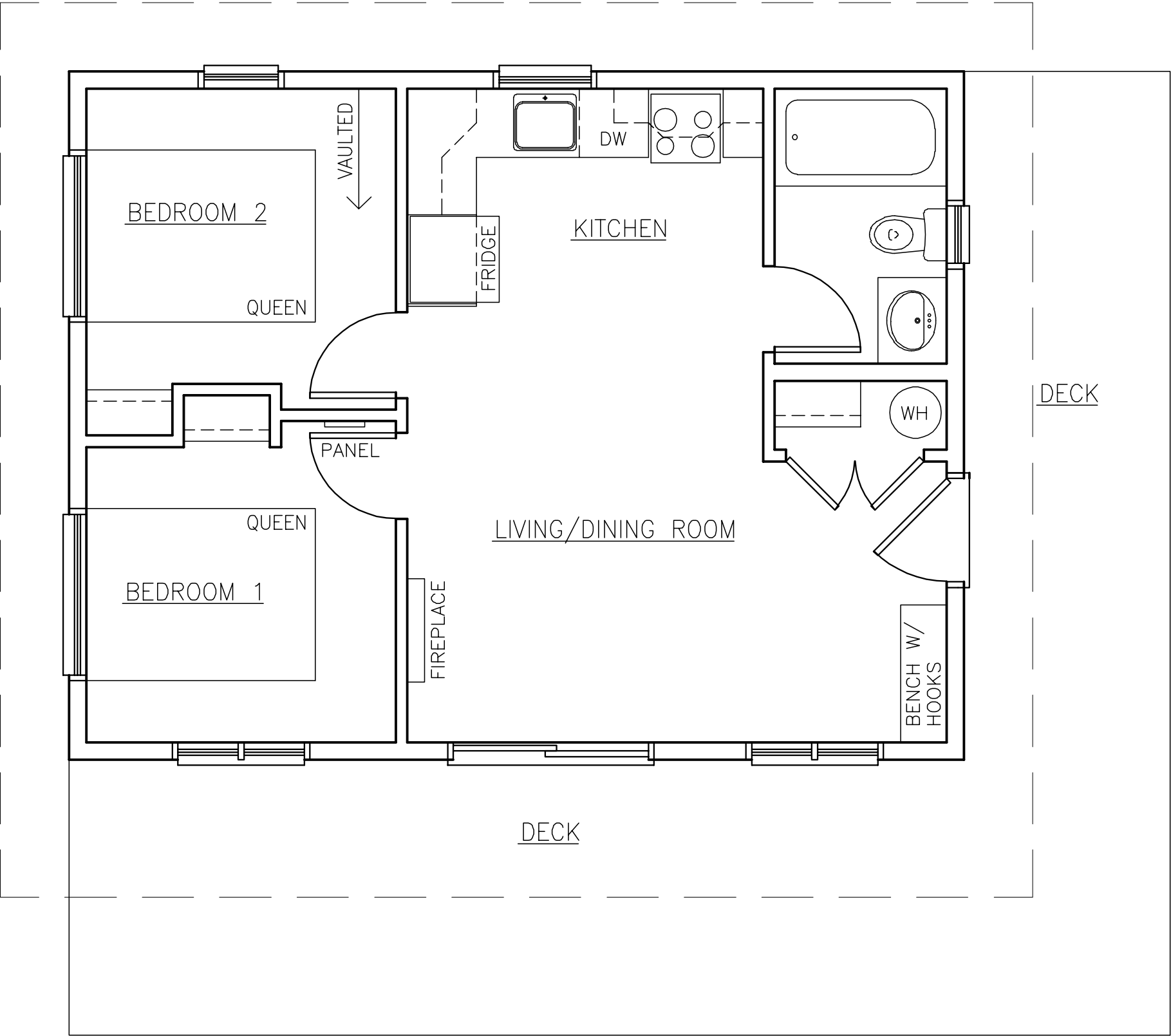
MAIN FLOOR PLAN 520 SQ.FT
